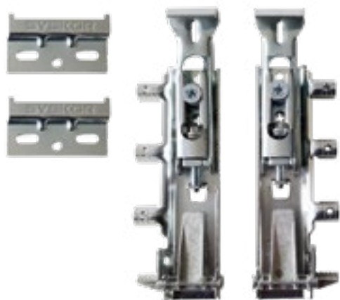
K HIDDEN HANGER SET ALPINE K65 Set of 1 bag with 2 hangers and 2 hooks
